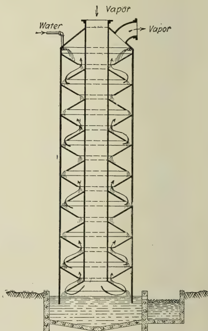
FIG. 64.—Baffle Scrubber.
